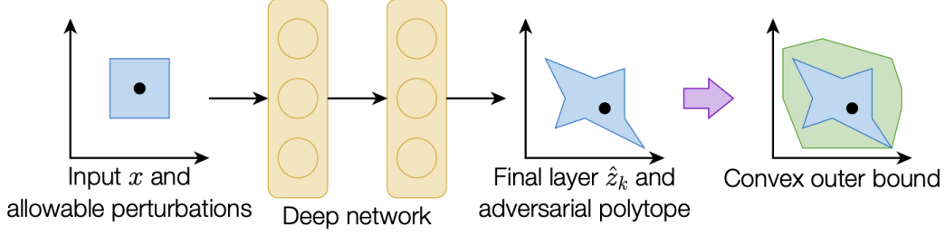
Figure 1: The non-convex adversarial polytope and its corresponding convex outer bound as shown in [4].
